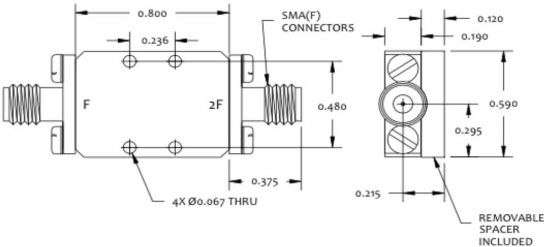
Outline drawing
